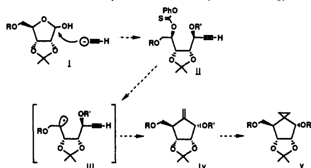
Scheme I. Schematic Representation of the Synthetic Strategy
