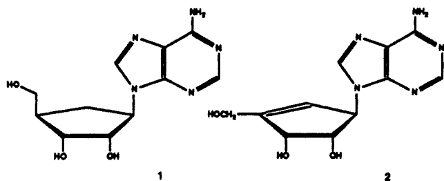
Scheme I. Schematic Representation of the Synthetic Strategy
