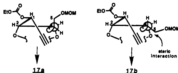
Scheme III. Illustration of Potential Steric Interactions That May Destabilize the Transition State Leading to 17b
